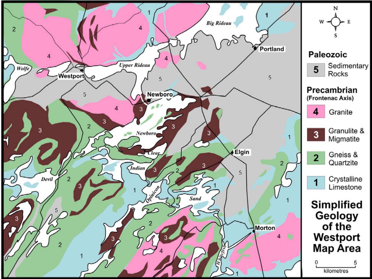
This highly simplified geology map shows some of the contact area between the Frontenac Axis (units 1, 2, 3 and 4) and the younger sedimentary rocks (unit 5) in the central Rideau area.
